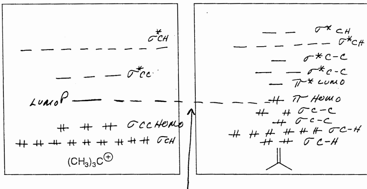
Molecular orbital energy level diagrams
